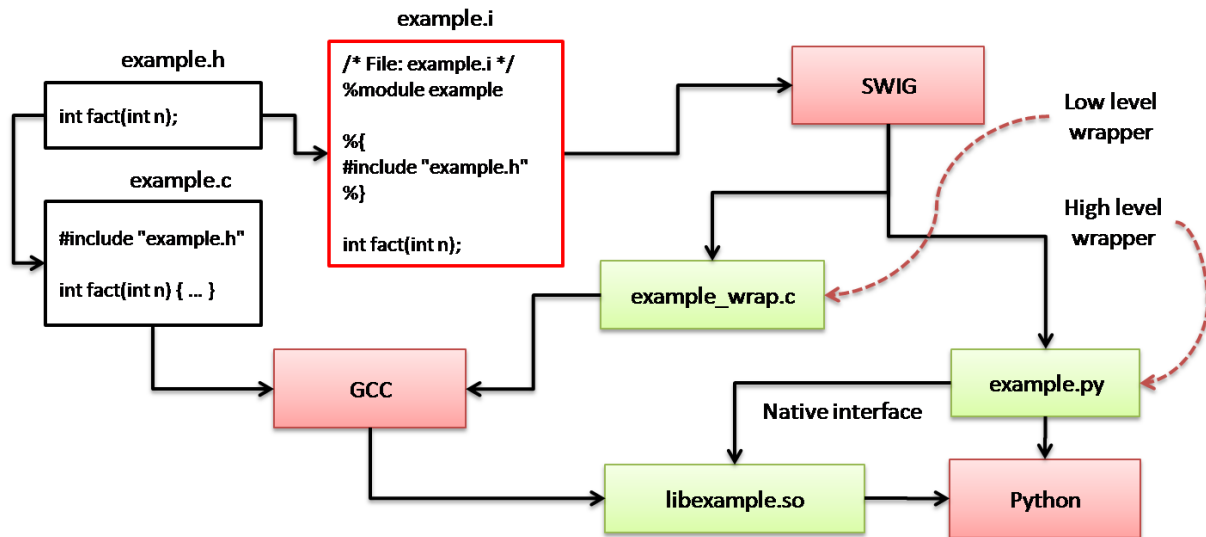
Figure 12. SWIG wrapping example
