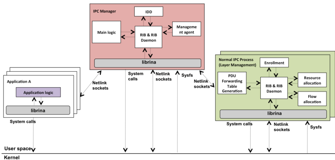
Figure 2. The IRATI user-space high level architecture [irati-ieee-network-magazine]
