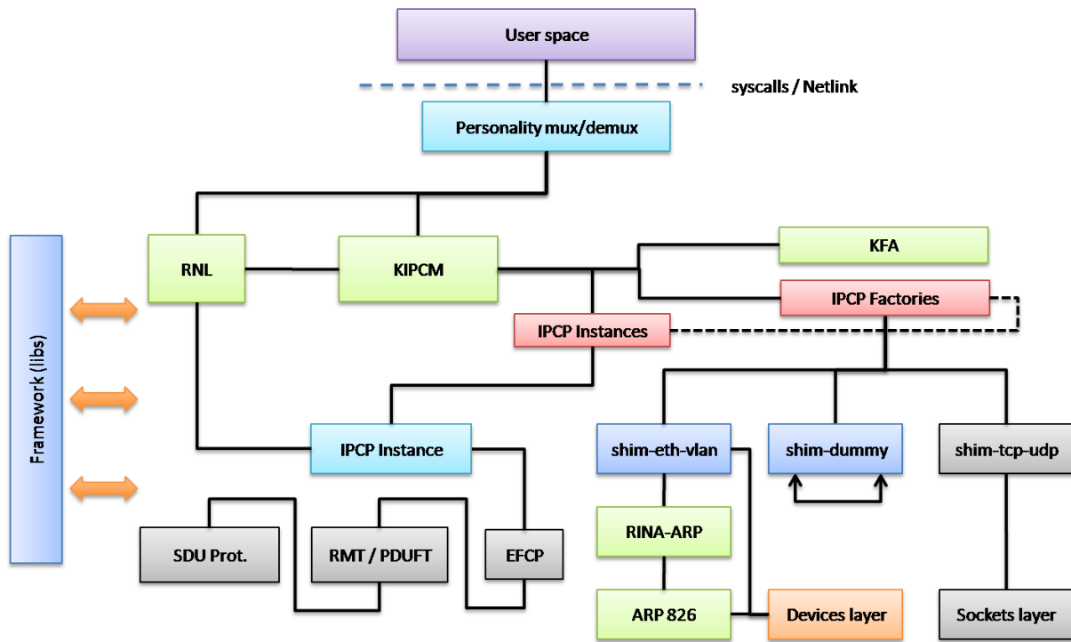
Figure 3. IRATI kernel-space high-level architecture
